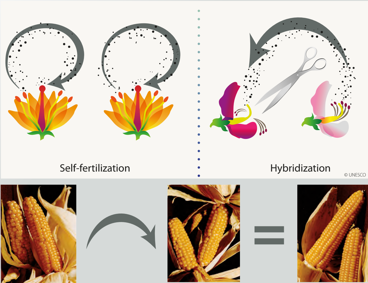
FIGURE 23: SELF-FERTILIZATION AND HYBRIDIZATION OF PLANTS
