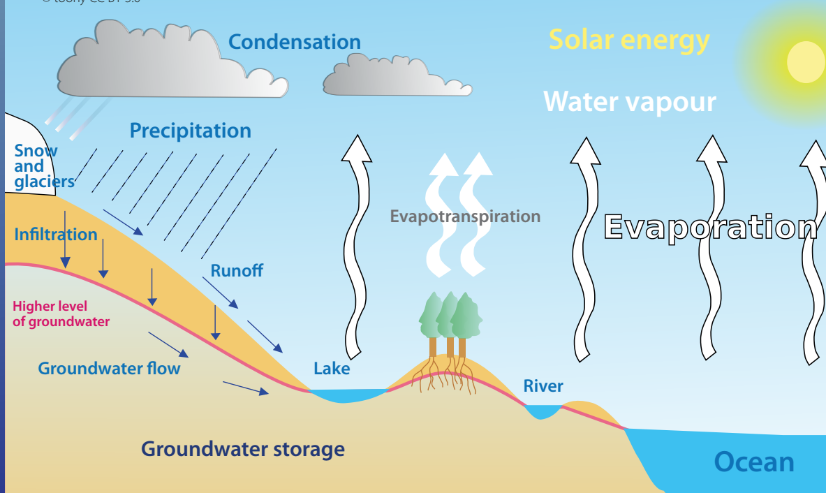
FIGURE 27: THE WATER CYCLE
