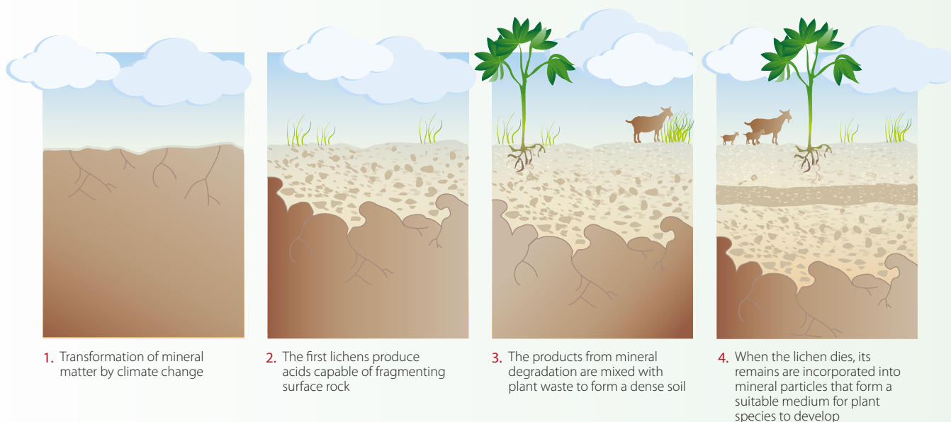
FIGURE 29: SOIL FORMATION
