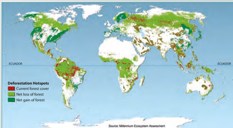
FIGURE 18: DEFORESTATION HOTSPOTS
